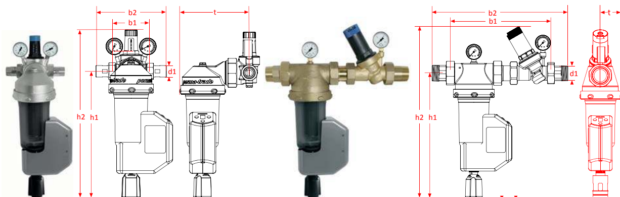
PT-FDK 40/50 A
